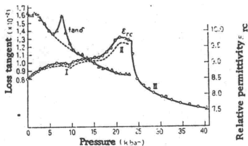
Fig. 6. Pressure dependence of relative permittivity ( \epsilon_{rc} ) and loss tangent ( \tan \delta ) of a c-plate \text{CaCO}_3 at 100 kHz (24°C).
